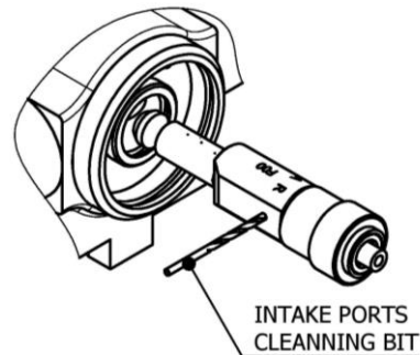
Cleaning Product Intake Holes Flat Chamber
