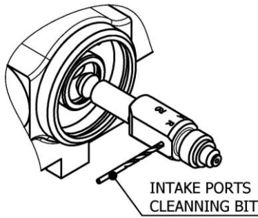
Cleaning Product Intake Holes Round Chamber
